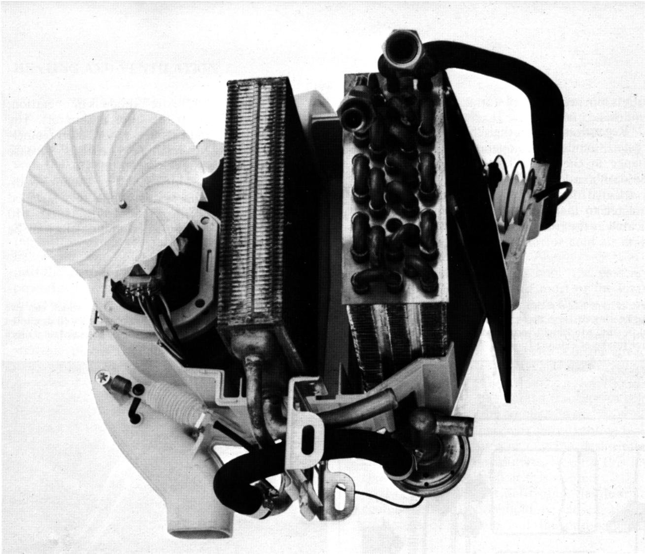
Exposed view of Volvo's new combined unit was taken from the side so only one of the two fans is shown. The heating core is in the center next to the evaporator unit for air conditioning. Because air passes through the evaporator before entering the heater core, moisture can be removed on damp winter days and the air then heated.
