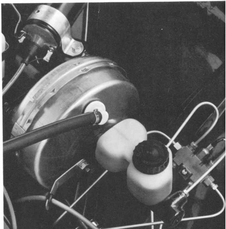
Hydraulic brake fluid level in the translucent twin reservoir can be inspected without removing the cap.
