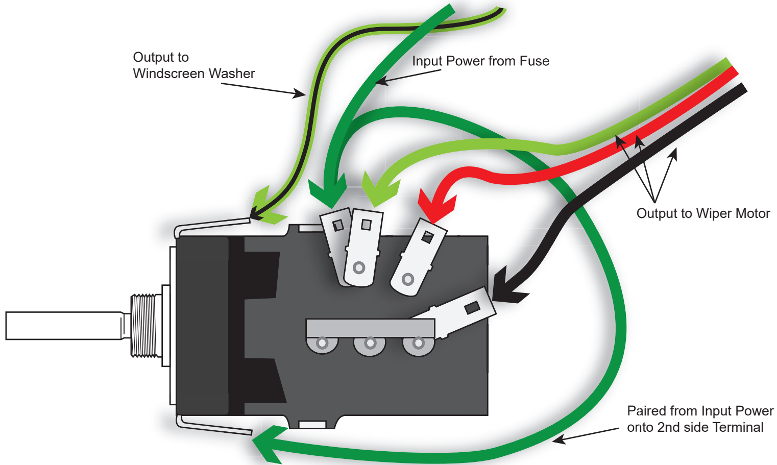
P1800 & 1800S Lucas Wiper Switch Terminals
