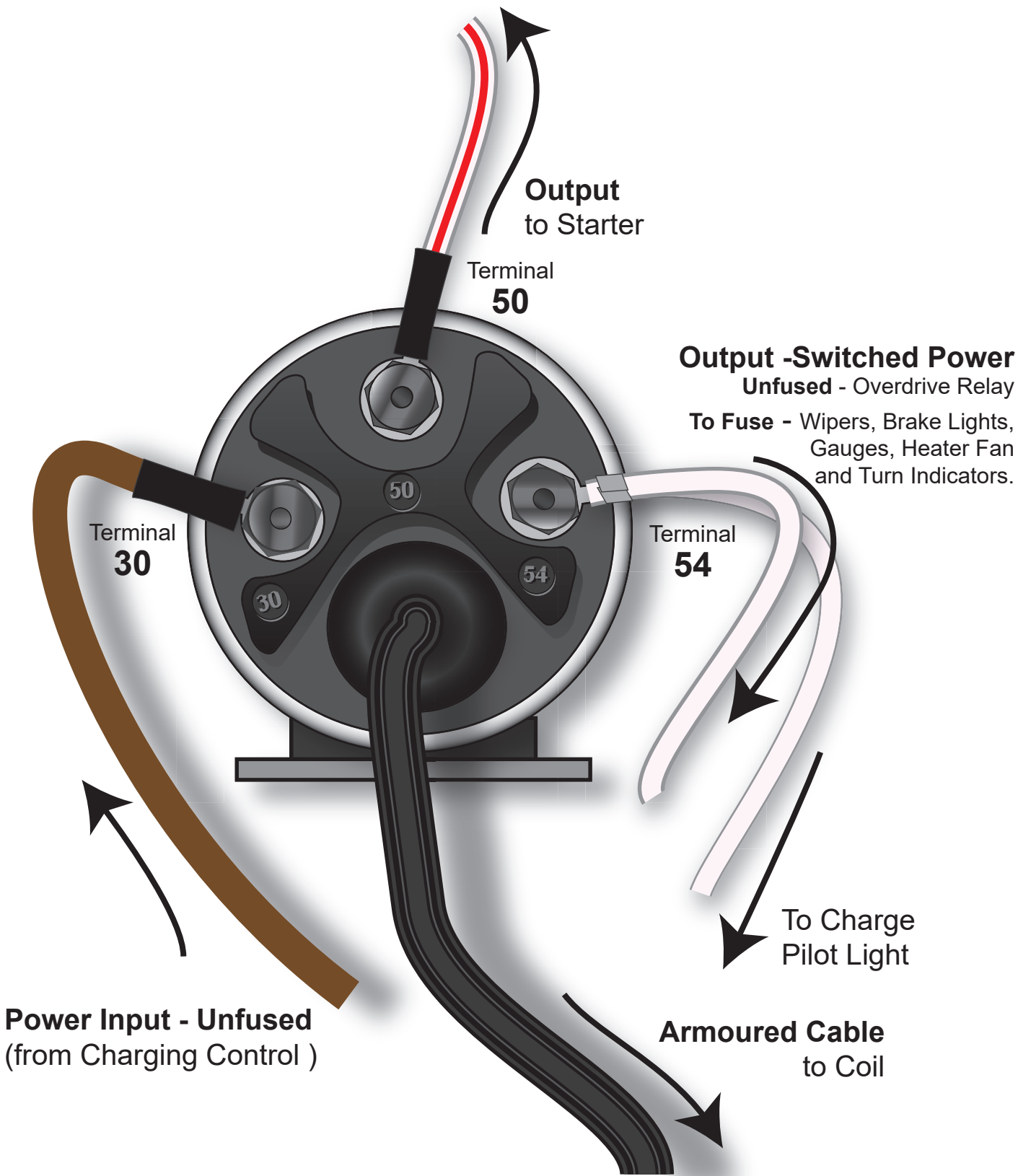
Ignition Switch Wiring Volvo P1800 & 1800 S 61 - 69
