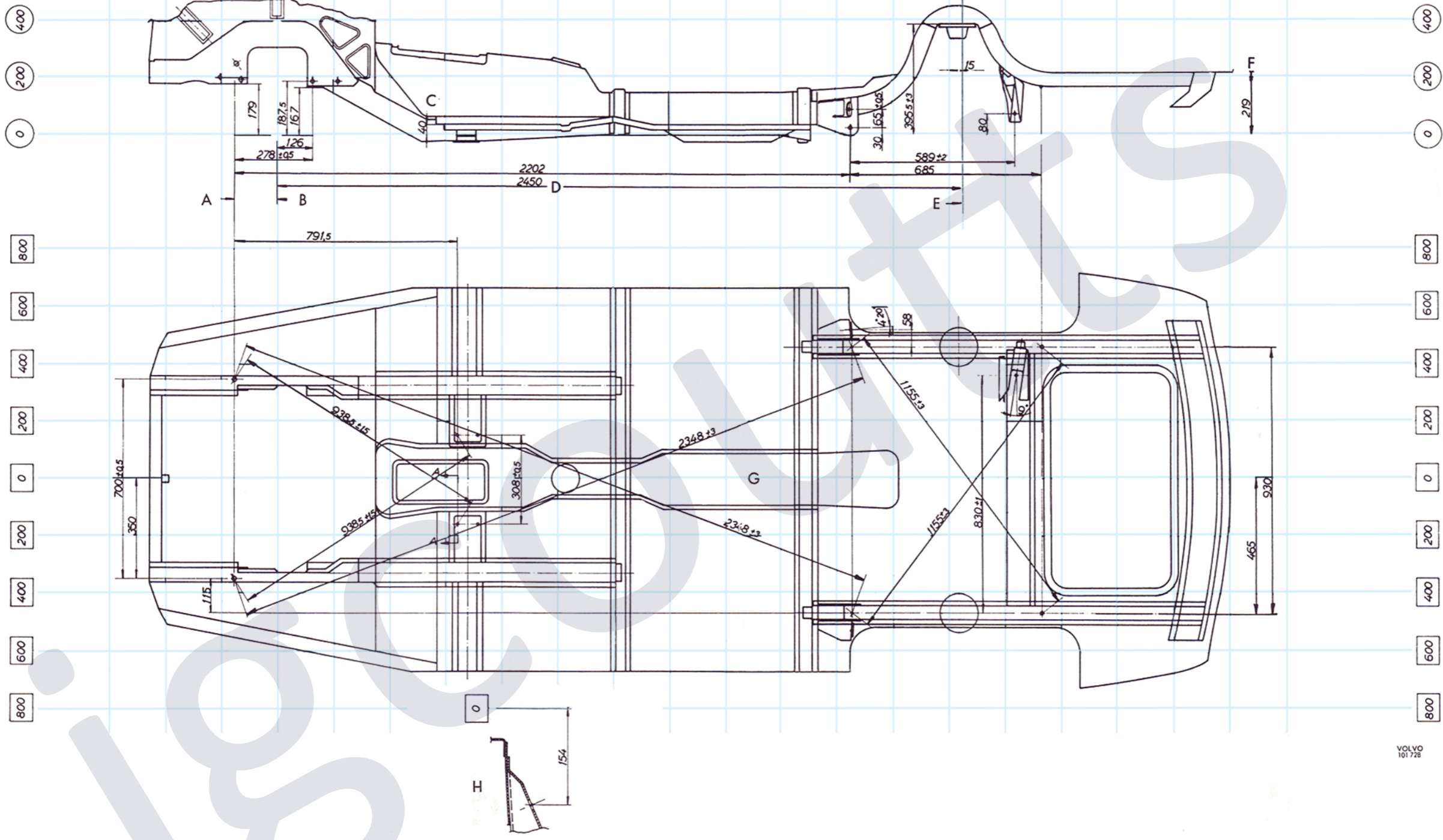
Plate A. Control drawing for body floor P 1800 up to chassis No. 16499.
